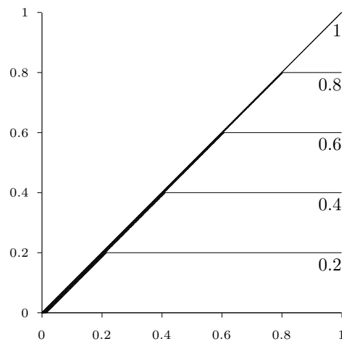
The Gödel t-norm
