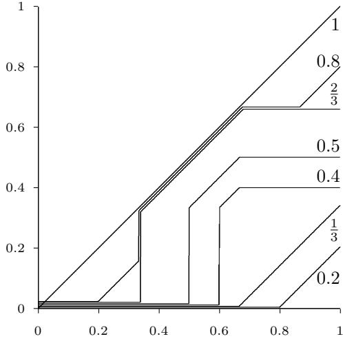
The rotation-annihilation of two Łukasiewicz t-norms
