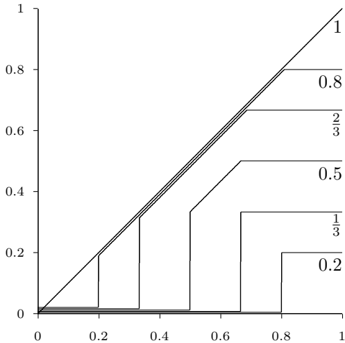
The t-norm J
