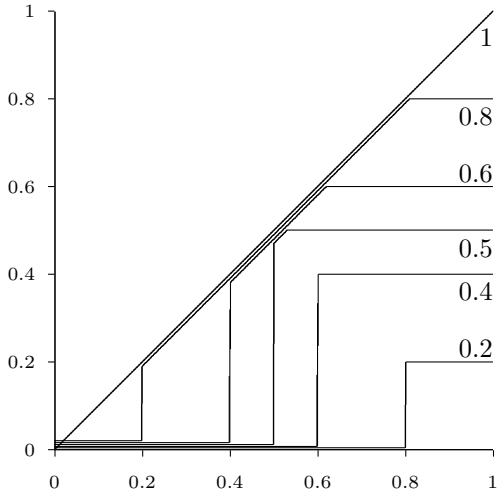
The nilpotent minimum t-norm
