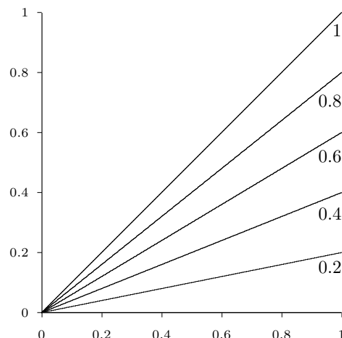
The product t-norm
