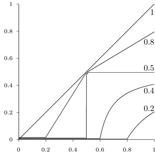
The rotated product t-norm
