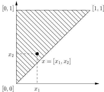
Figure 1: The lattice \mathcal{L}^I
