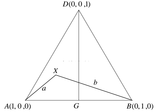
Figure 2: The triangle ABD (cf. Fig. 1) explaining a distance-based measure of fuzziness
